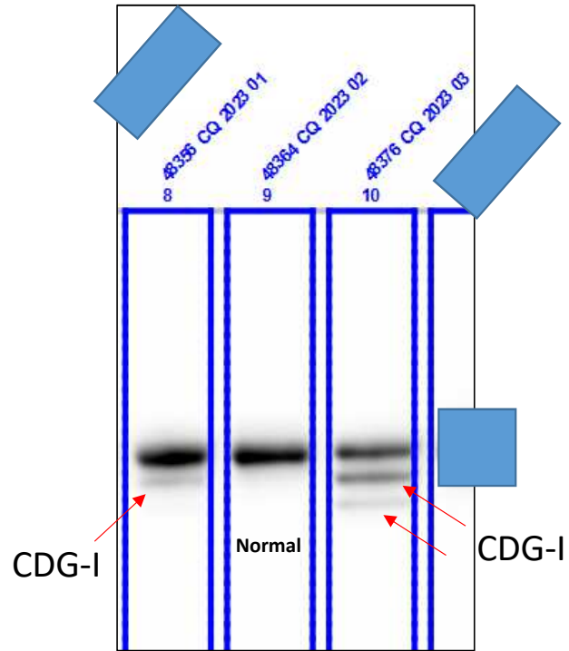
EEQ ERNDIM CDG-PP-2023 A/B/C Western blot of transferrin
